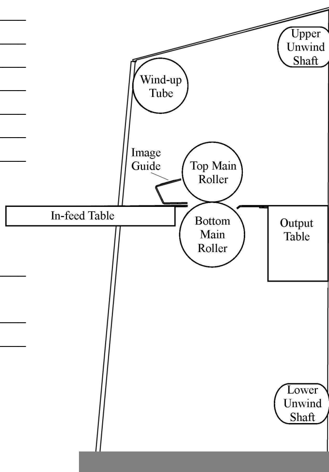
Figure 25: Blank Webbing Diagram
