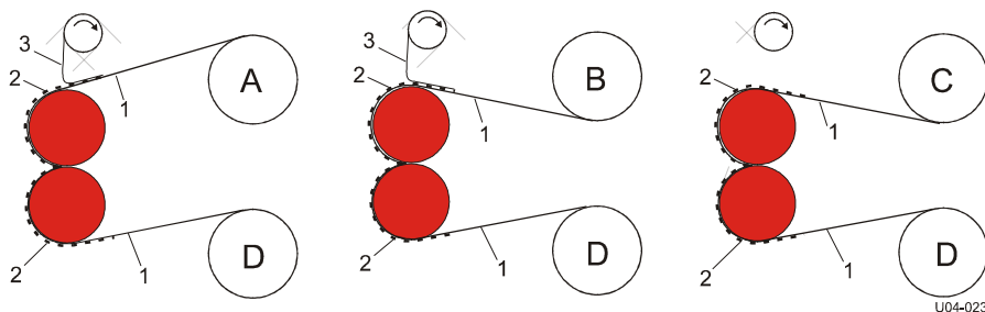
Figure 14: Film adhesives.
