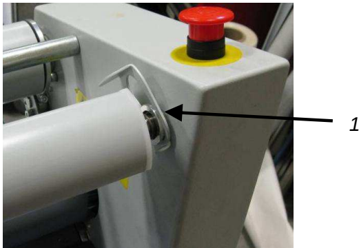
Figure 11: Interlock up
